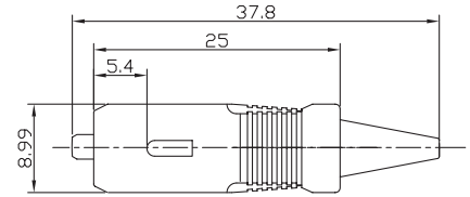
Hood Type 0.9mm
